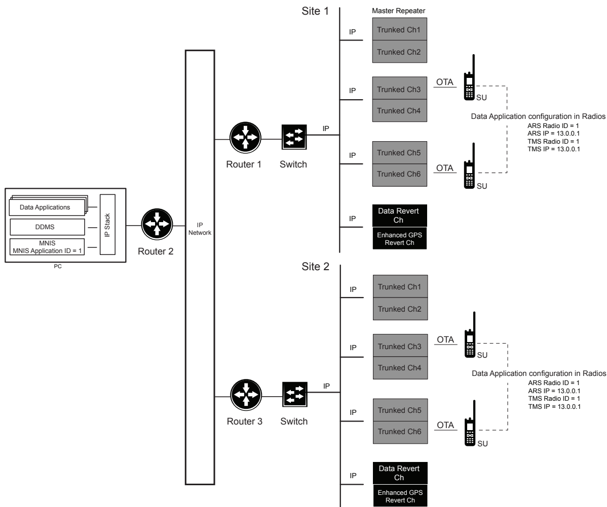
Figure 179: Capacity Plus Multi Site System with MNIS
