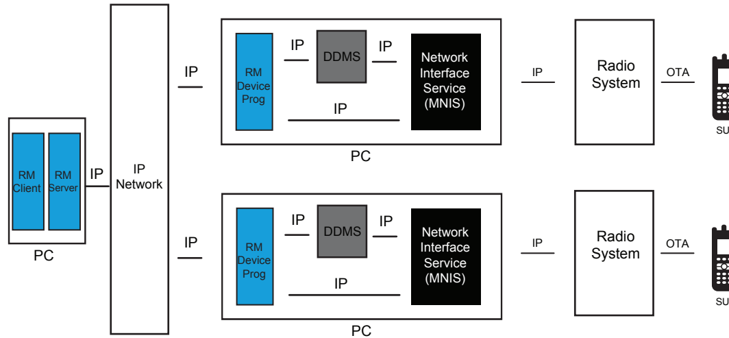
Figure 62: RM Server with Remote RM Device Programmers and MNIS
