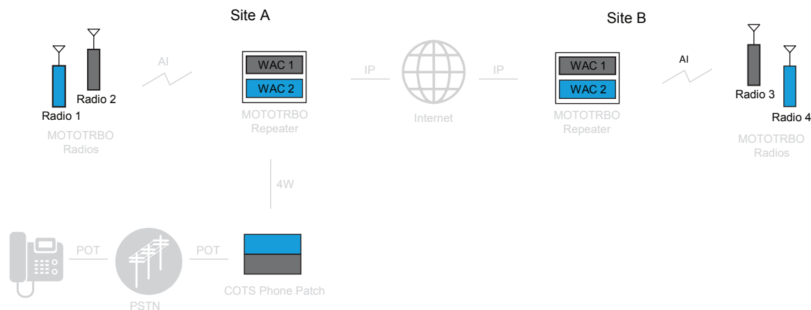
Figure 67: One APP Box Supporting Two Wide Area Channels in IP Site Connect
