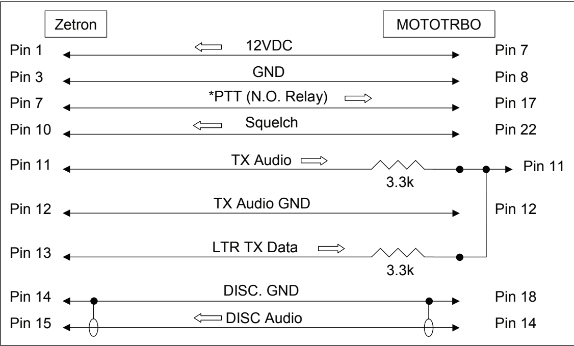
Figure 74: XPR 8300/XPR 8380/XPR 8400 Cable Schematic for Zetron Controllers
