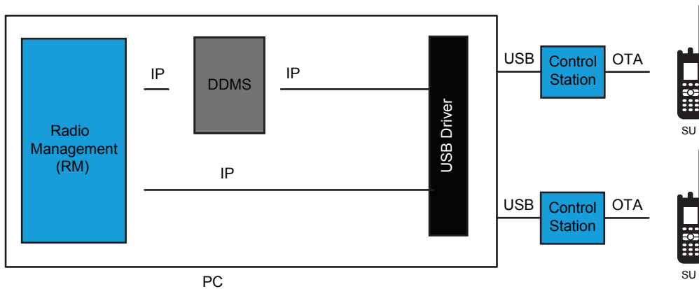
Figure 192: Multi-Channel RM Application with Control Stations in Single Site Repeater Mode
