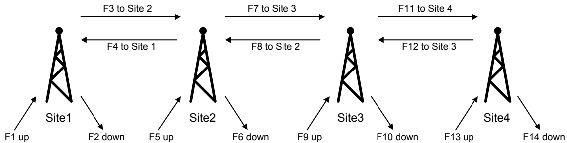
Figure 219: Example of a Dedicated MOTOTRBO Link System with Four Backhaul Sites
