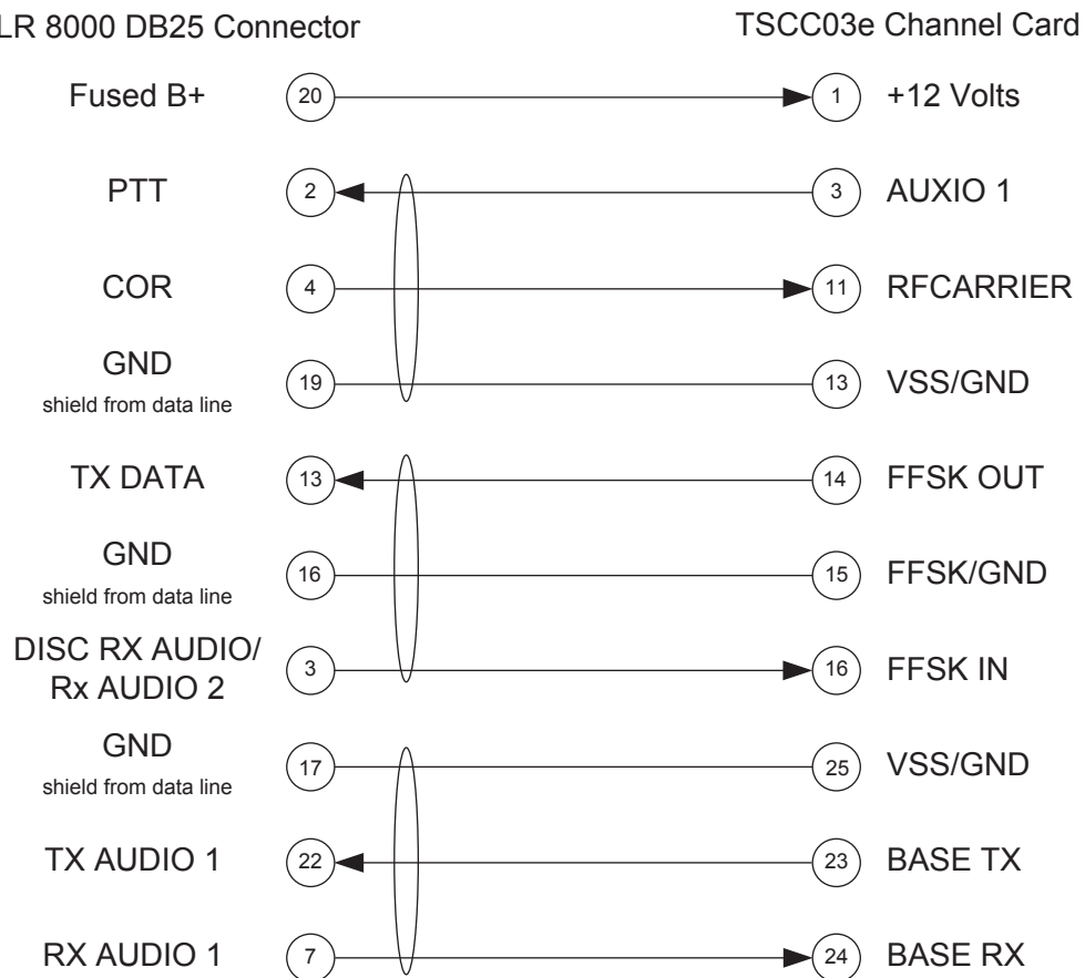
Figure 78: Hardware Connections between SLR 5000/SLR 8000 and TSCC03 Channel Controller
