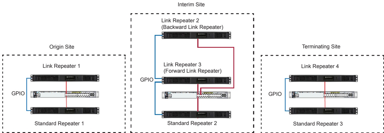
Figure 11: MOTOTRBO Link System: Example 2
