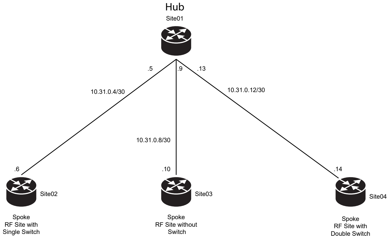
Figure 231: Hub-to-Spoke VPN Overlay Tunnel Network
