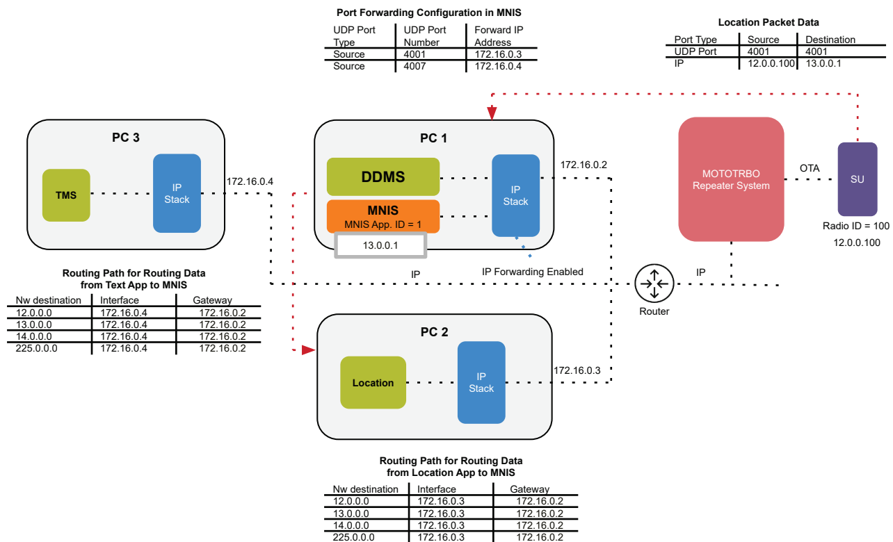
Figure 182: Application and MNIS Deployed on Separate PCs
