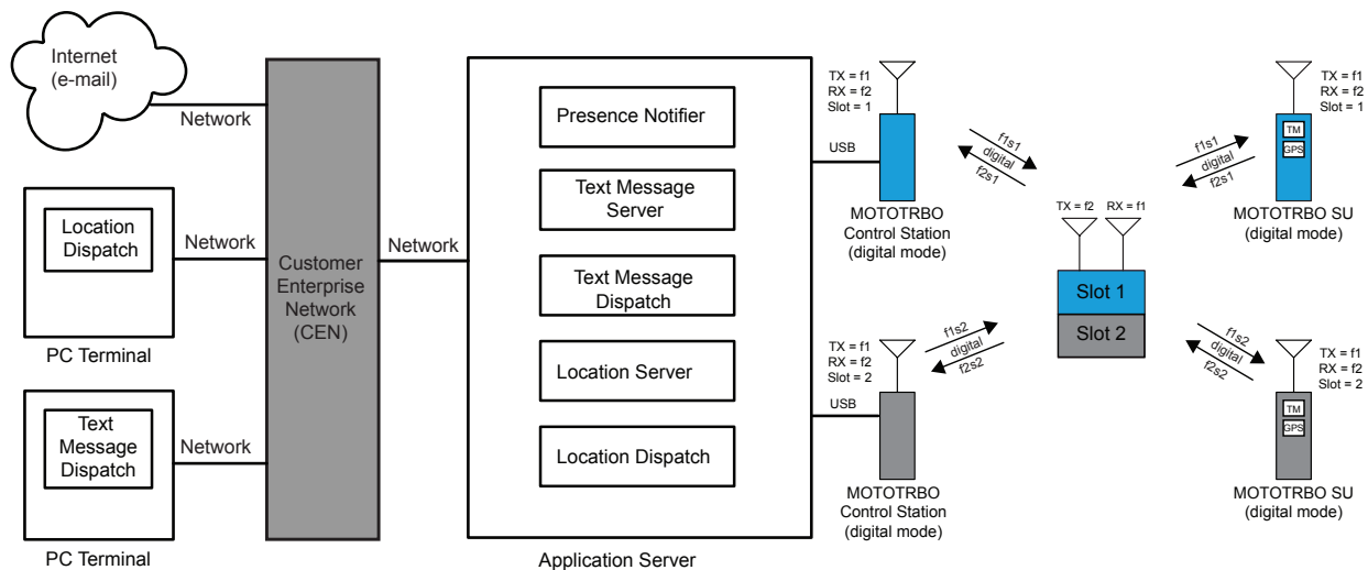
Figure 114: MOTOTRBO Radios in Digital Two-Slot Digital Repeater Mode with a Server-Based Configuration Using Control Stations and Remote Dispatchers
