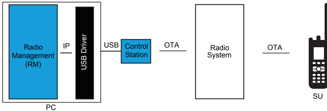
Figure 52: Single Channel Non-Remote RM Configuration Through Control Station
