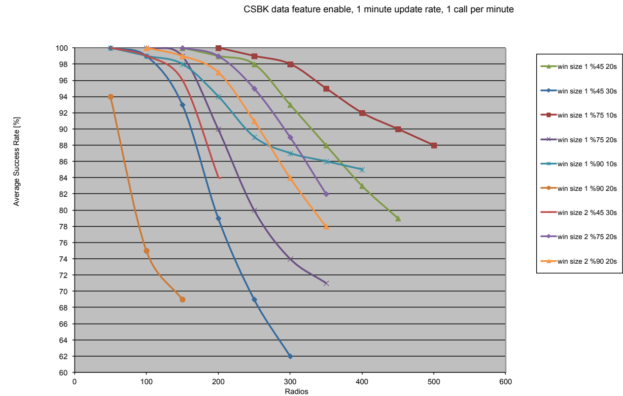
Figure 156: 1-Minute Update Rate with Different Window Sizes, Loading and Call Duration
