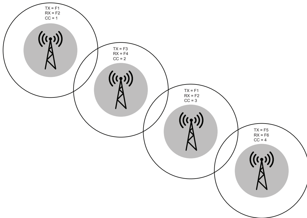
Figure 31: Corridor Coverage
