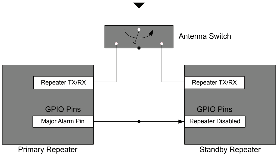
Figure 35: Redundant Repeater Setup
