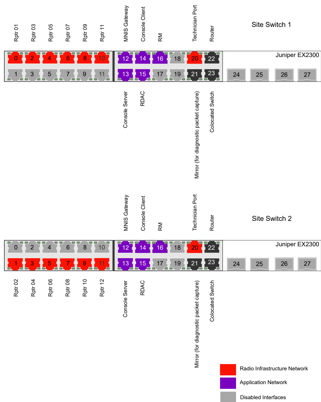
Figure 230: Ports and VLANs Assignment on a Juniper EX 2300 Switch in Repeater Site with a Double Switch
