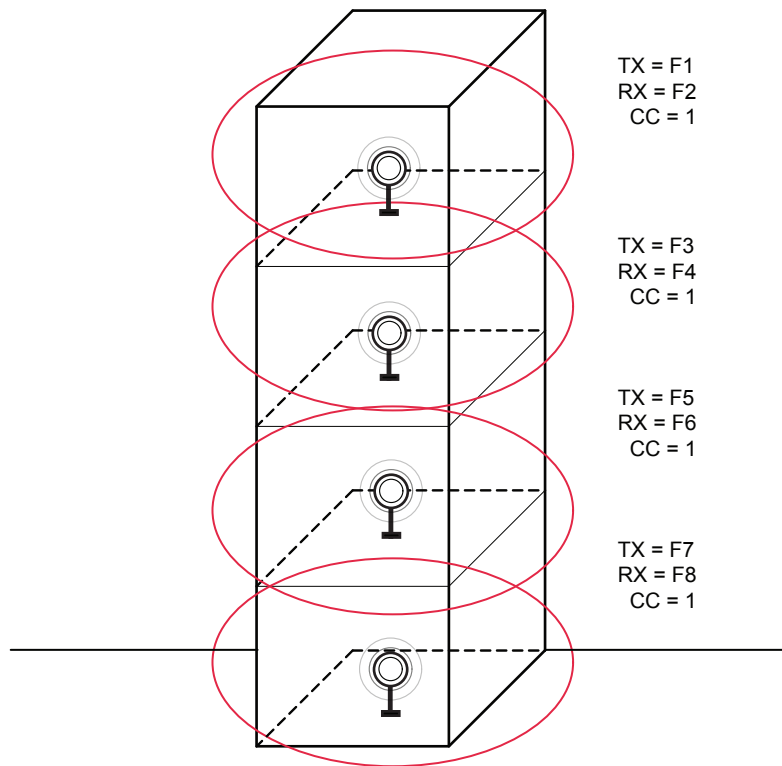
Figure 32: Multi-Floor Coverage
